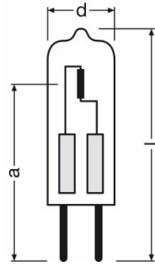
HALOSTAR 24 V 50 W 24 V GY6.35, HALOSTAR 24 V 100 W 24 V GY6.35
